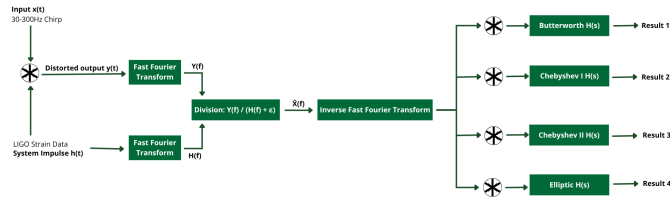
Figure 1. Block diagram detailing the complete signal modeling and recovery.
